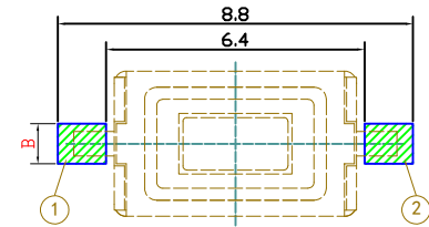
P. C. B MOUNTING PATTERN DIMENSION the following soldering are recommended for reflow soldering
